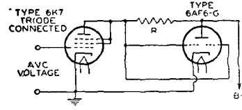
R: TYPICAL VALUE IS 0.5 MEGOHM
