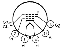
12D ULTOR = G_3 + CL
