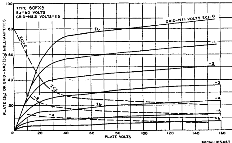
AVERAGE CHARACTERISTICS
