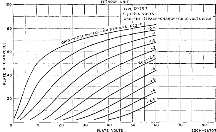
AVERAGE CHARACTERISTICS TETRODE UNIT
