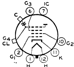
12C ULTOR = G_4 + CL FOCUSING ELECTRODE = G_3
