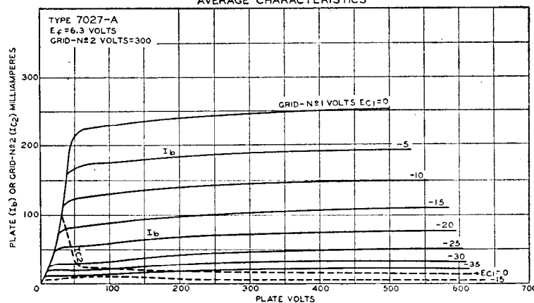
AVERAGE CHARACTERISTICS
