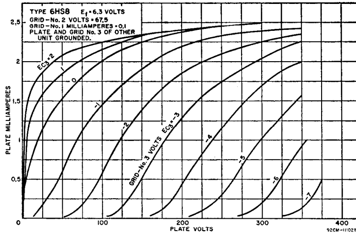
AVERAGE CHARACTERISTICS
