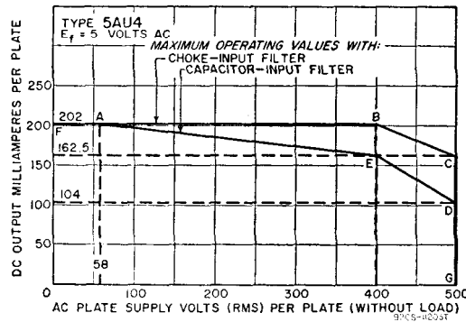
RATING CHART
