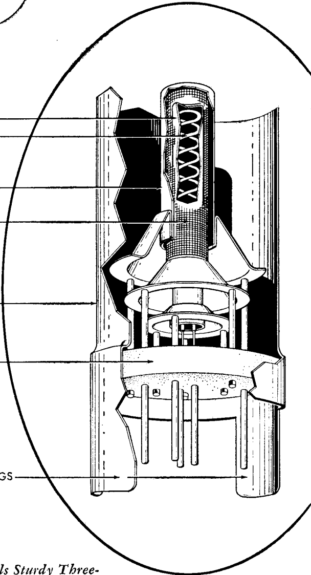
Cut-Away Reveals Sturdy Three-Point Support Of Cylindrical Electrodes
