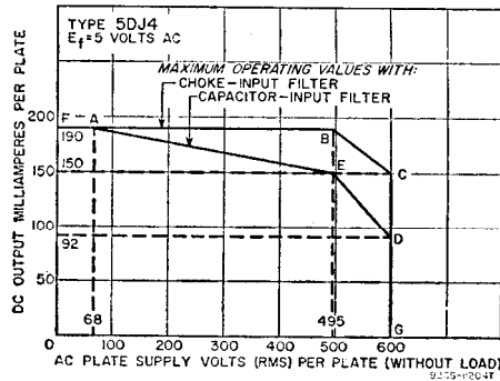
RATING CHART
