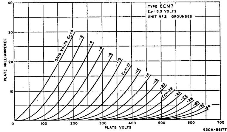
AVERAGE CHARACTERISTICS UNIT N°1
