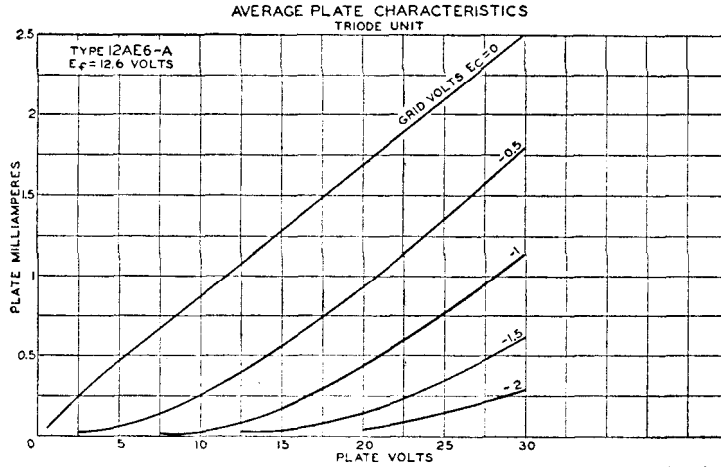
Characteristics of 12AE6-A with 12.6 Volts on Heater:
